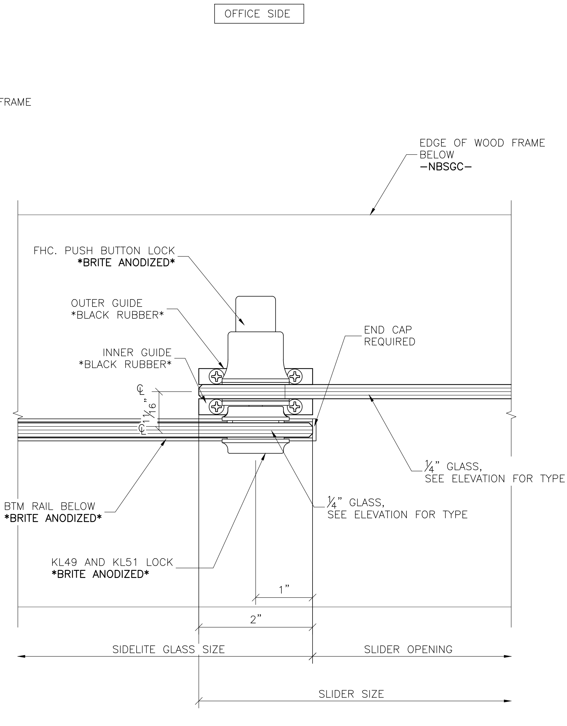
V2 PASS THRU WINDOW SIDELITE-DOOR DETAIL ARCH REF: NONE
